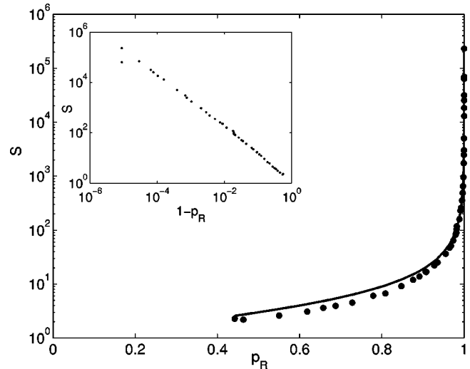
FIG. 4. Mean avalanche size S as a function of p_R : experimental data (points) and model (solid line). For the experimental data, p_R has been estimated as N_b / (N_b + N_j) , where N_b is the total number of fallen beads and N_j the total number of jamming, for a given orifice size. Inset: the same data, plot in logarithmic scale as a function of 1 - p_R .
