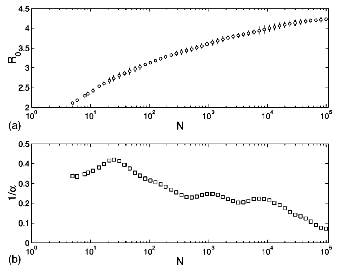
FIG. 3. (a) R_0 vs N . Note the logarithmic scale on the horizontal axis. (b) 1/\alpha as a function of N in semilogarithmic scale. Both R_0 and \alpha were obtained from the fits of Fig. 2.
