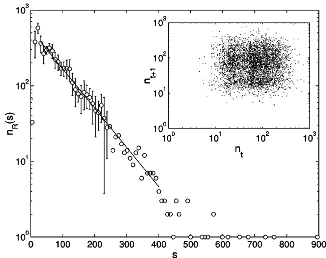
FIG. 1. Histogram for the number of grains that flow between two successive jammings. Data correspond to R=3 (the beads have a diameter of 2 mm, and the circular orifice is 6 mm wide). More than 4000 events have been recorded. The line is a linear fit. Inset: first return map, i.e., the avalanche size n_t vs the next avalanche size n_{t+1} . Note that t is just a correlative index ordering the sequence of avalanches.
