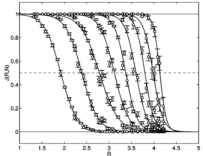
FIG. 2. Jamming probability J as a function of R . Each series corresponds to a fixed N , i.e., the probability of the orifice getting jammed before N grains pass through it. Data taken for several bead diameters are displayed. Successive series, from left to right, correspond to N=3, 10, 30, 100, 300, 1000, 3000, 10\,000 , and 30\,000 beads. The fit corresponds to a hyperbolic tangent with two adjustable parameters: J(R,N) = \{1 - \tanh[\alpha(R - R_0)]\}/2 . The two parameters of this family of curves, \alpha and R_0 , are shown in Fig. 3. Error bars are statistical.
